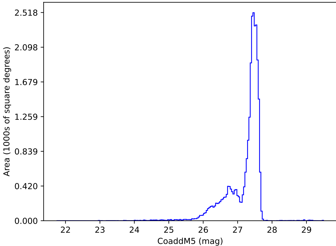
internal_u_expt27_nscale1.2v3.4_10yrs : CoaddM5
