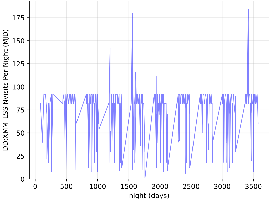
internal_u_expt27_nscale1.2v3.4_10yrs all bands: DD:XMM_LSS Nvisits Per Night
