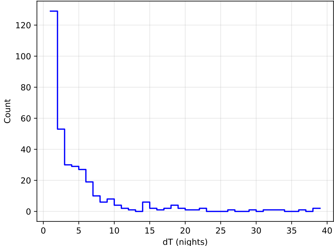
internal_u_expt27_nscale1.2v3.4_10yrs all bands: DD:WFD Delta Nights Histogram
