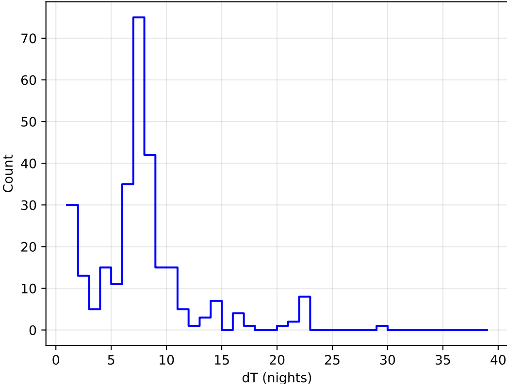
internal_u_expt27_nscale1.2v3.4_10yrs all bands: DD:EDFS Delta Nights Histogram
