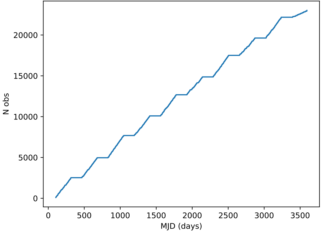
internal_u_expt27_nscale1.2v3.4_10yrs all bands: DD:EDFS Cumulative NVisits
