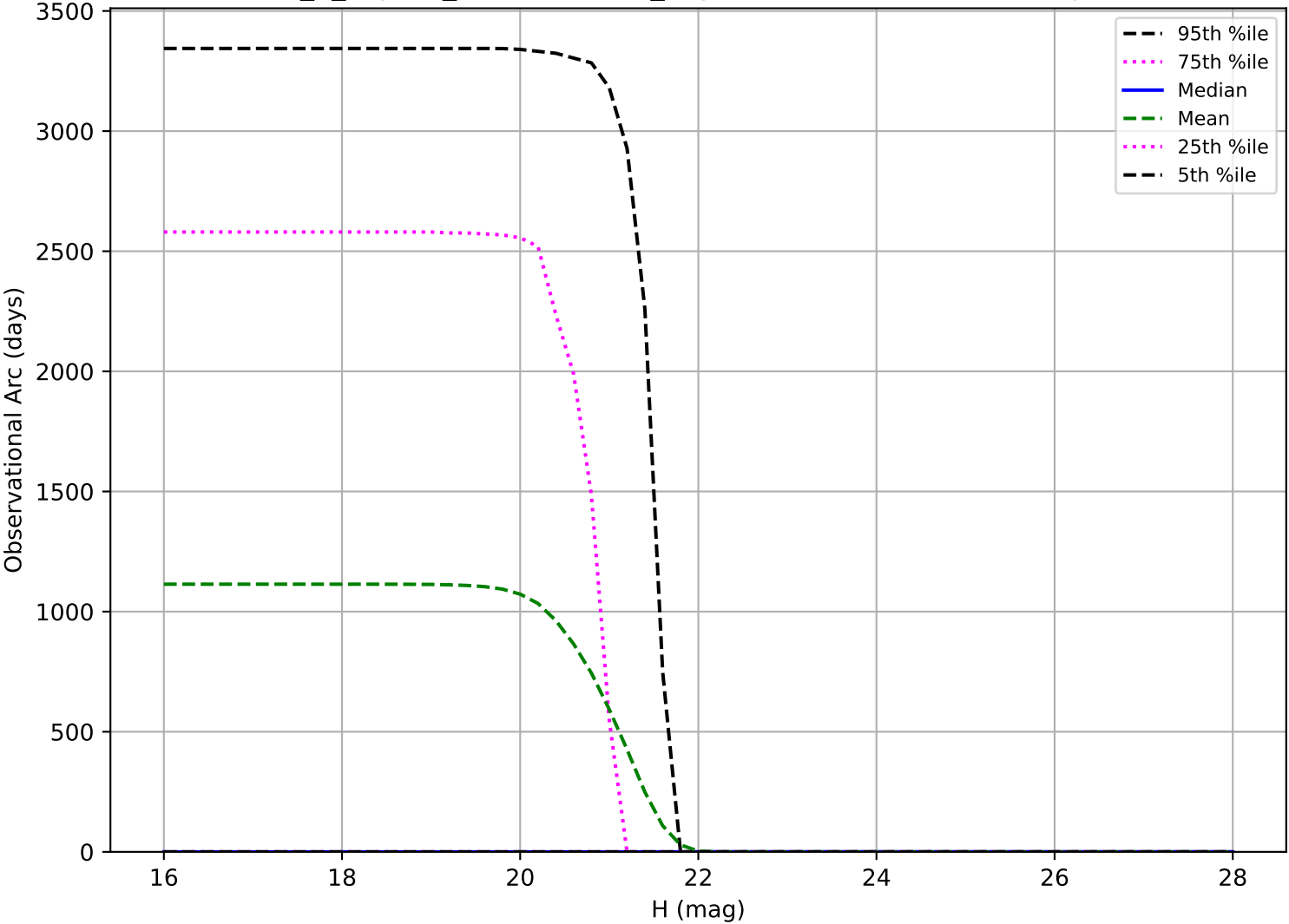
internal_u_expt27_nscales1.1v3.4_10yrs: Observational Arc Length Vatra
