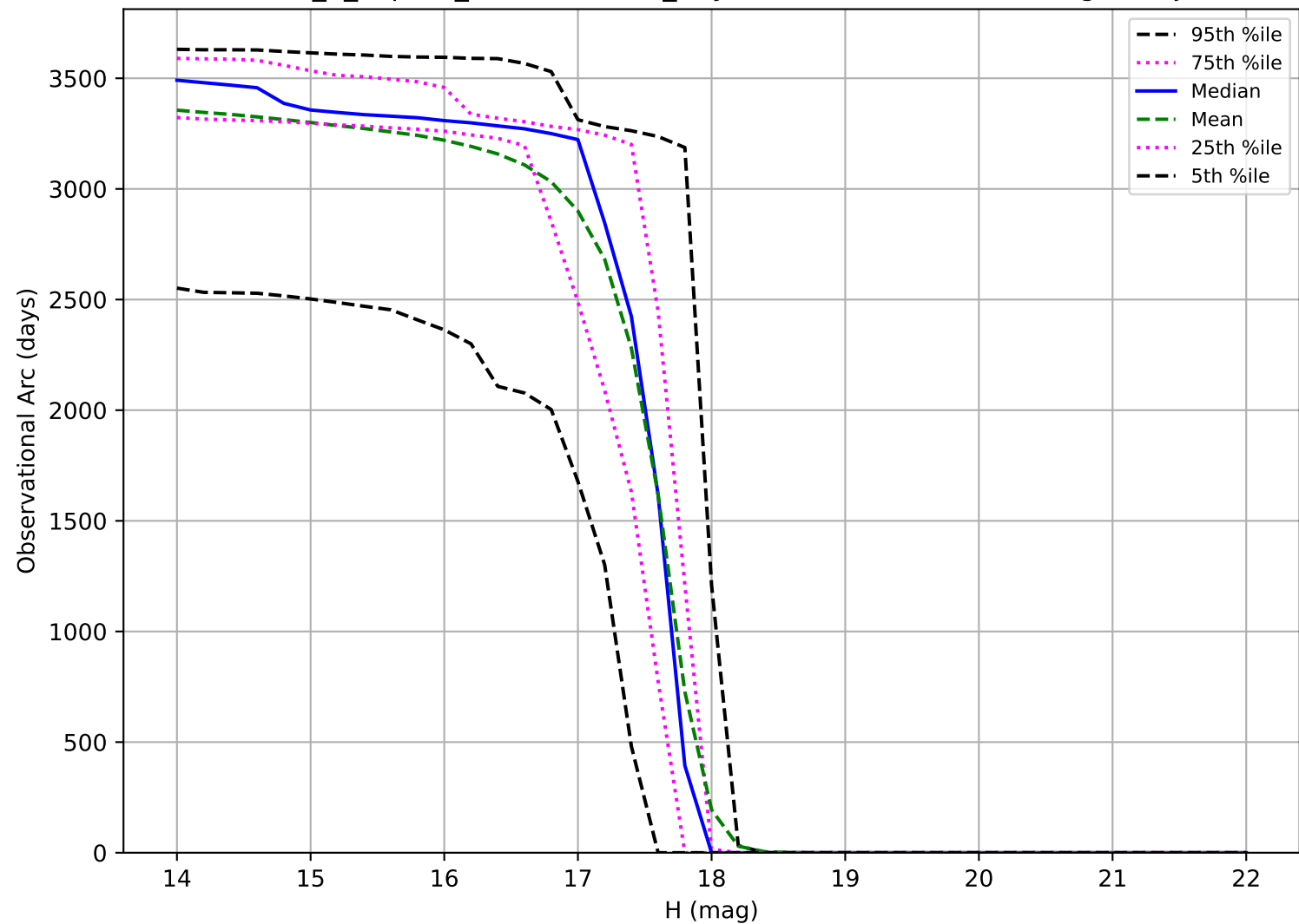
internal_u_expt27_nscale1.1v3.4_10yrs: Observational Arc Length Trojan
