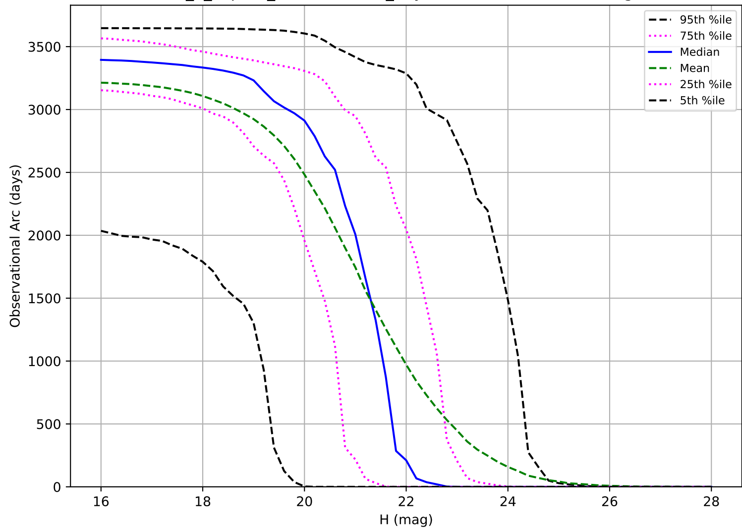
internal_u_expt27_nscale1.1v3.4_10yrs: Observational Arc Length PHA
