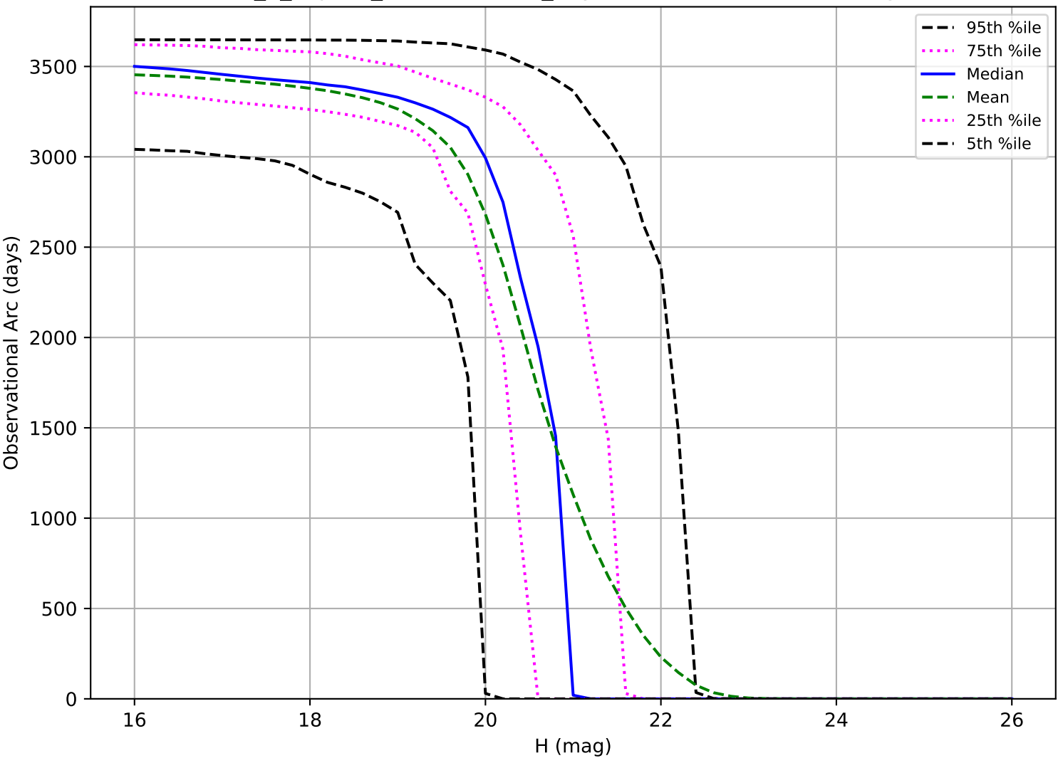
internal_u_expt27_nscales1.1v3.4_10yrs: Observational Arc Length MBA
