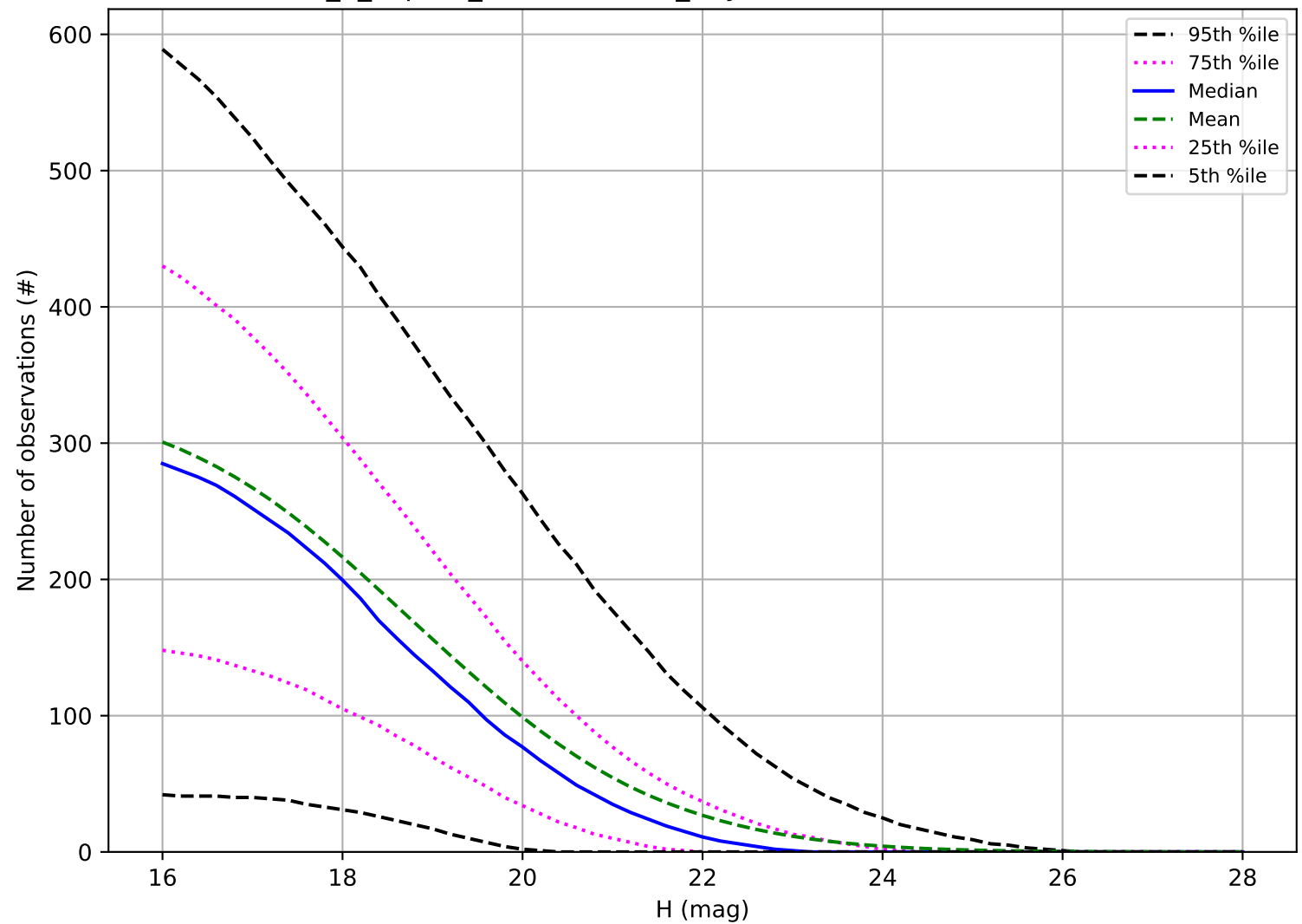
internal_u_expt27_nscale1.1v3.4_10yrs: Number of observations PHA
