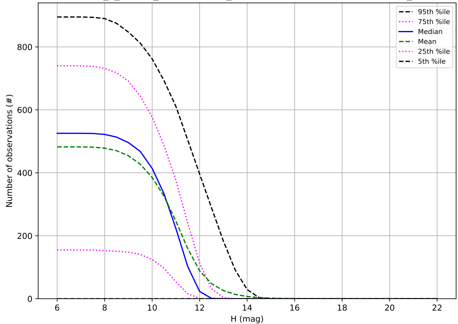
internal_u_expt27_nscale1.1v3.4_10yrs: Number of observations OCC_r20
