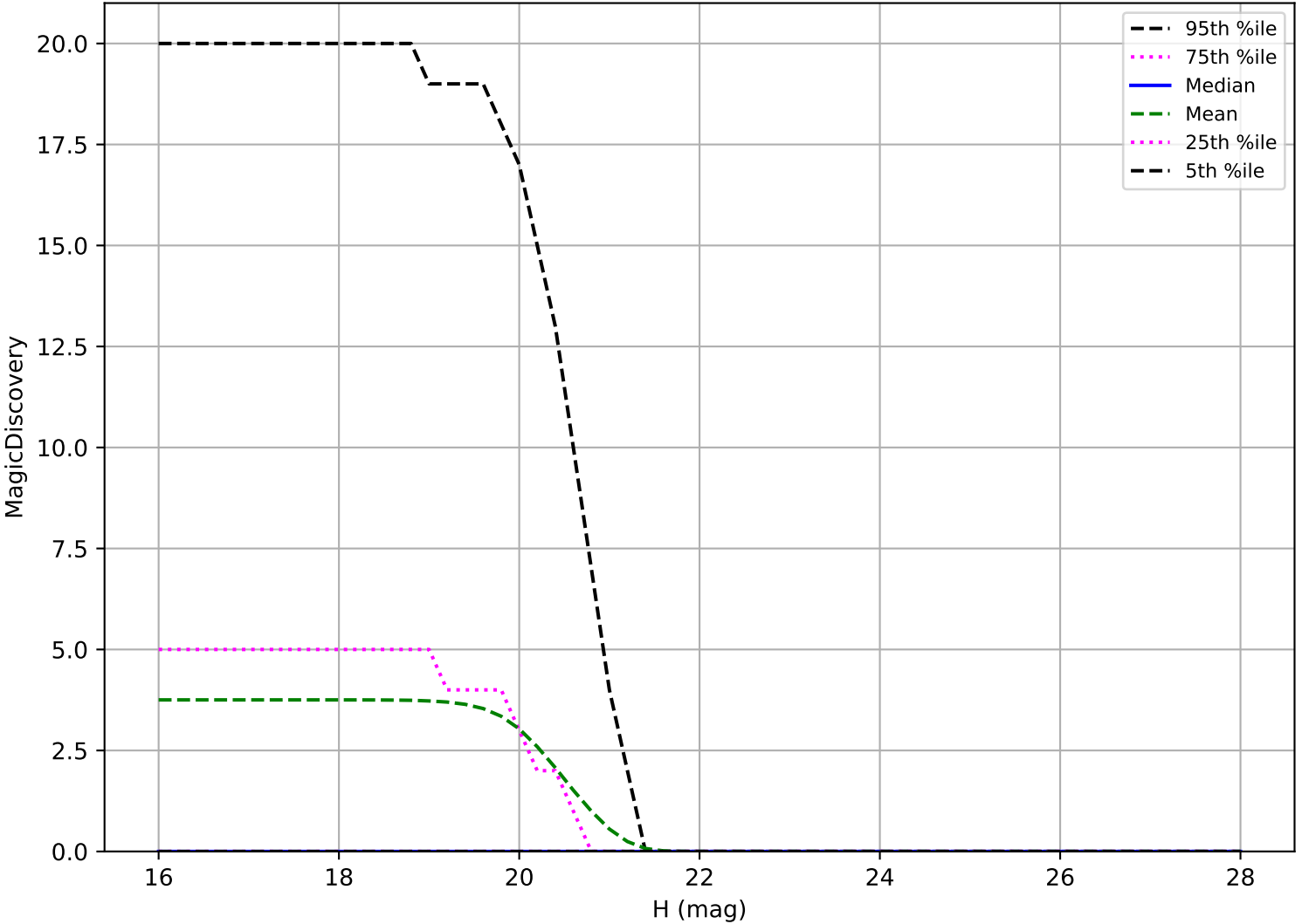
internal_u_expt27_nscale1.1v3.4_10yrs: Vatira 6 detections in 60 nights detection loss
