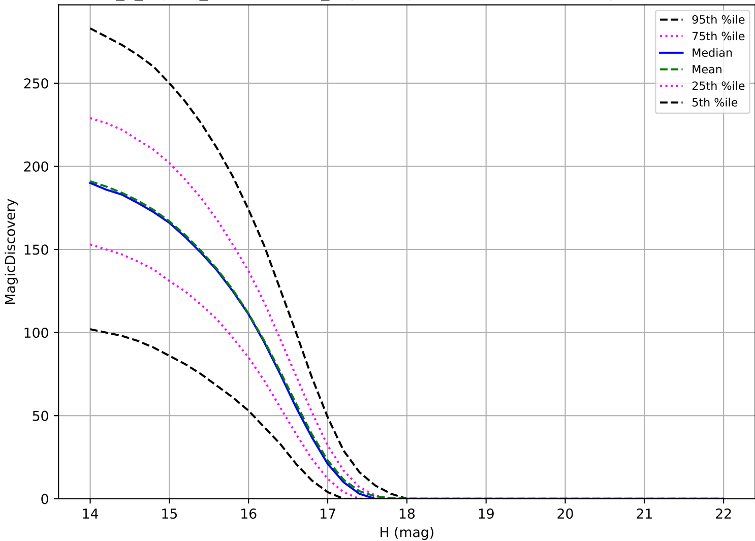
internal_u_expt27_nscale1.1v3.4_10yrs: Trojan 6 detections in 60 nights detection loss
