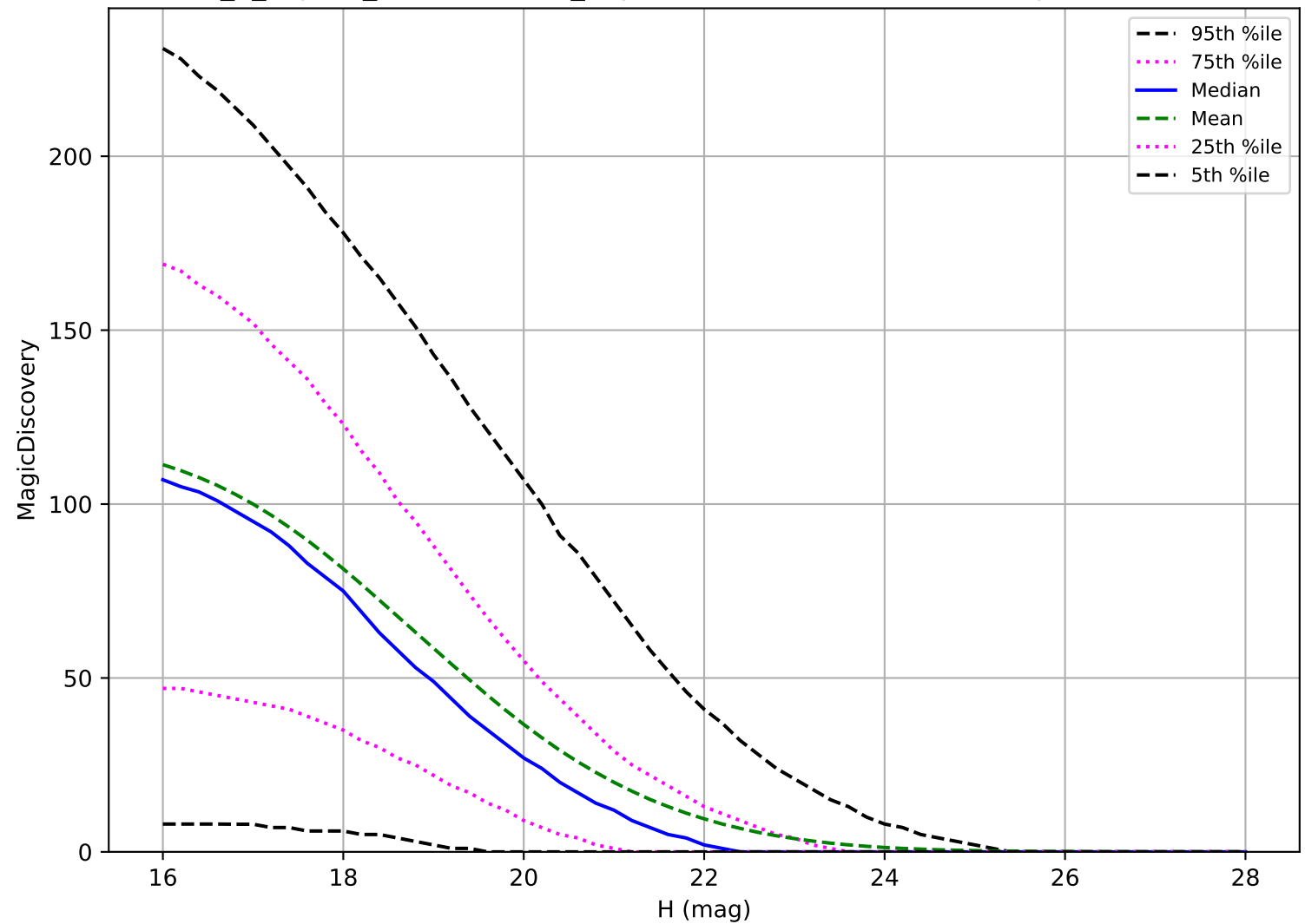
internal_u_expt27_nscale1.1v3.4_10yrs: PHA 6 detections in 60 nights detection loss
