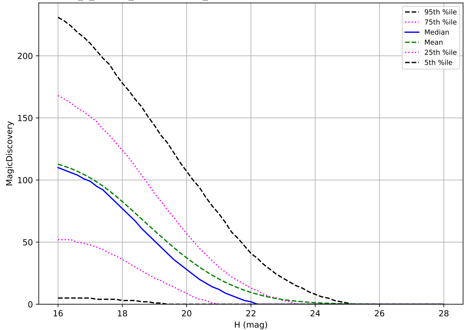
internal_u_expt27_nscale1.1v3.4_10yrs: NEO 6 detections in 60 nights detection loss
