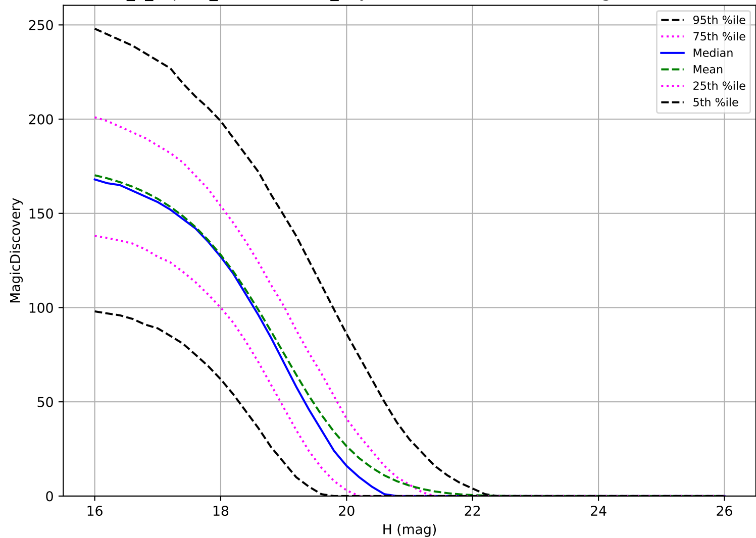
internal_u_expt27_nscale1.1v3.4_10yrs: MBA 6 detections in 60 nights detection loss
