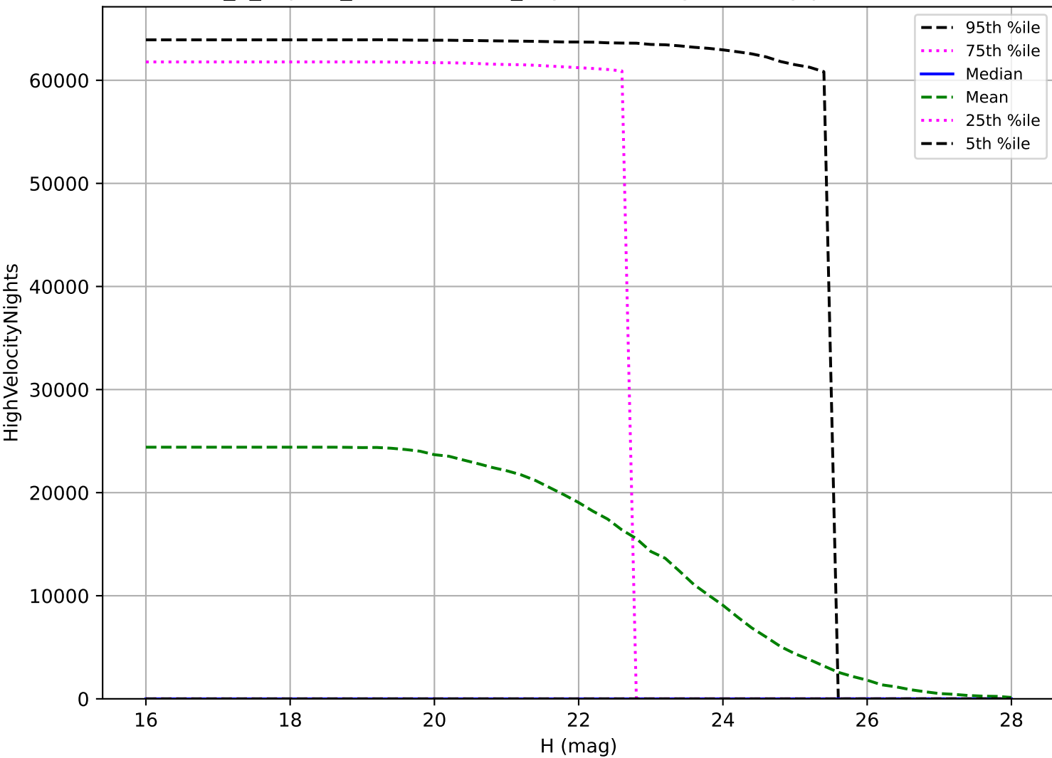
internal_u_expt27_nscale1.1v3.4_10yrs: PHA High velocity pair detection loss
