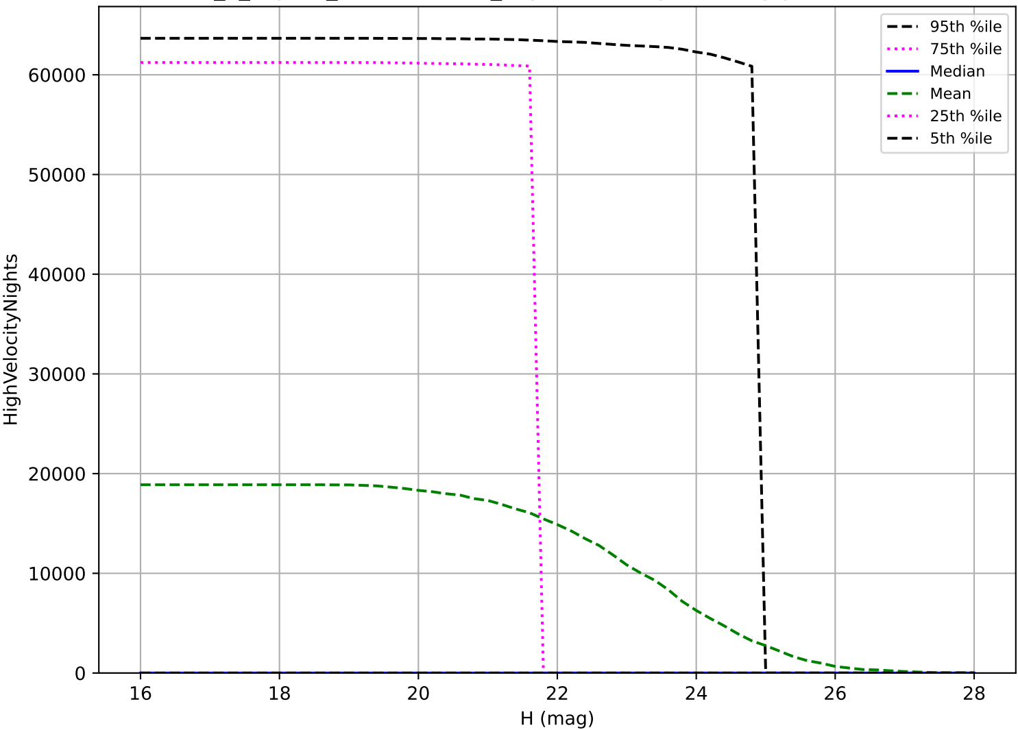
internal_u_expt27_nscale1.1v3.4_10yrs: NEO High velocity pair detection loss
