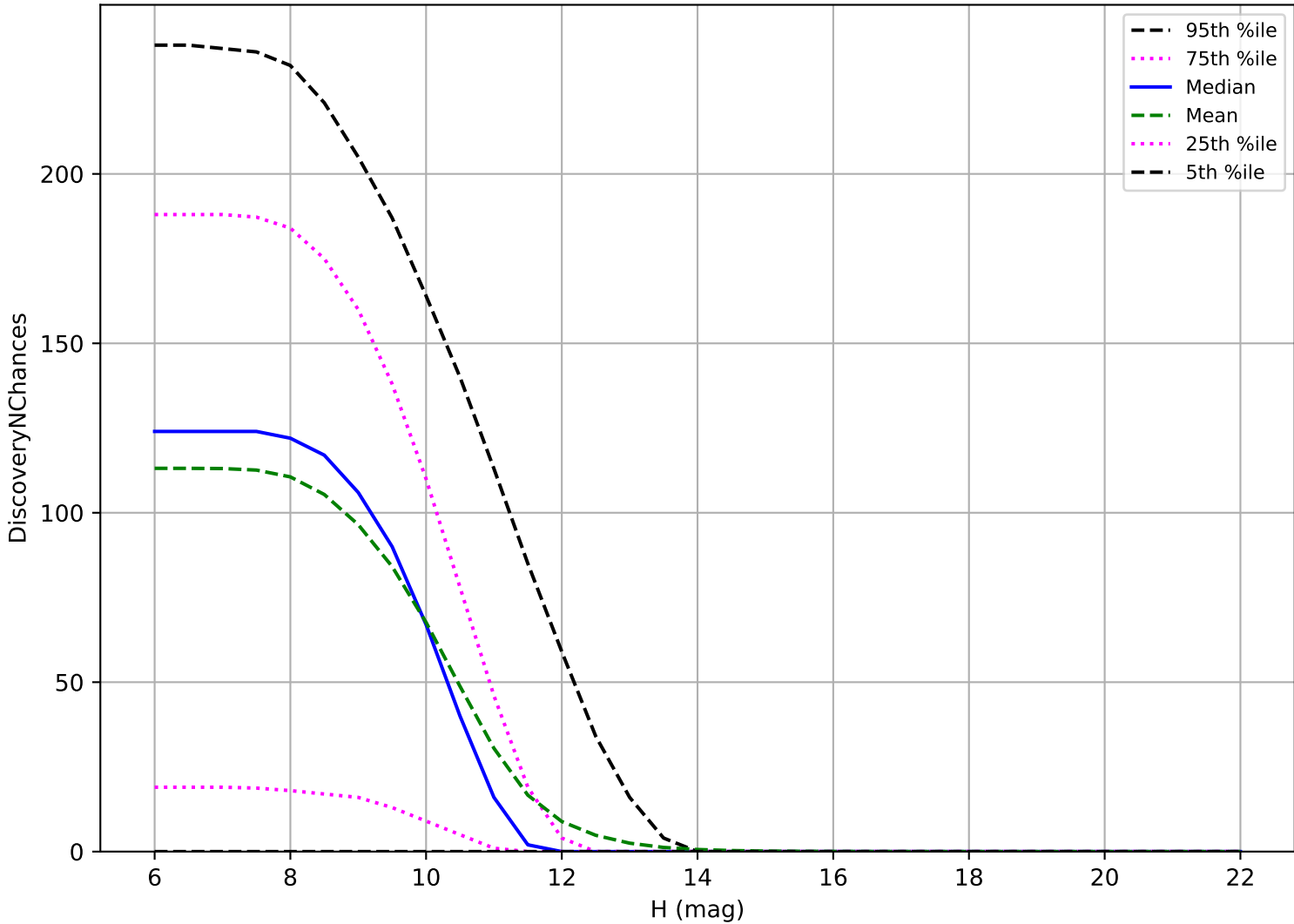
internal_u_expt27_nscale1.1v3.4_10yrs: OCC_r20 3 pairs in 15 nights detection loss
