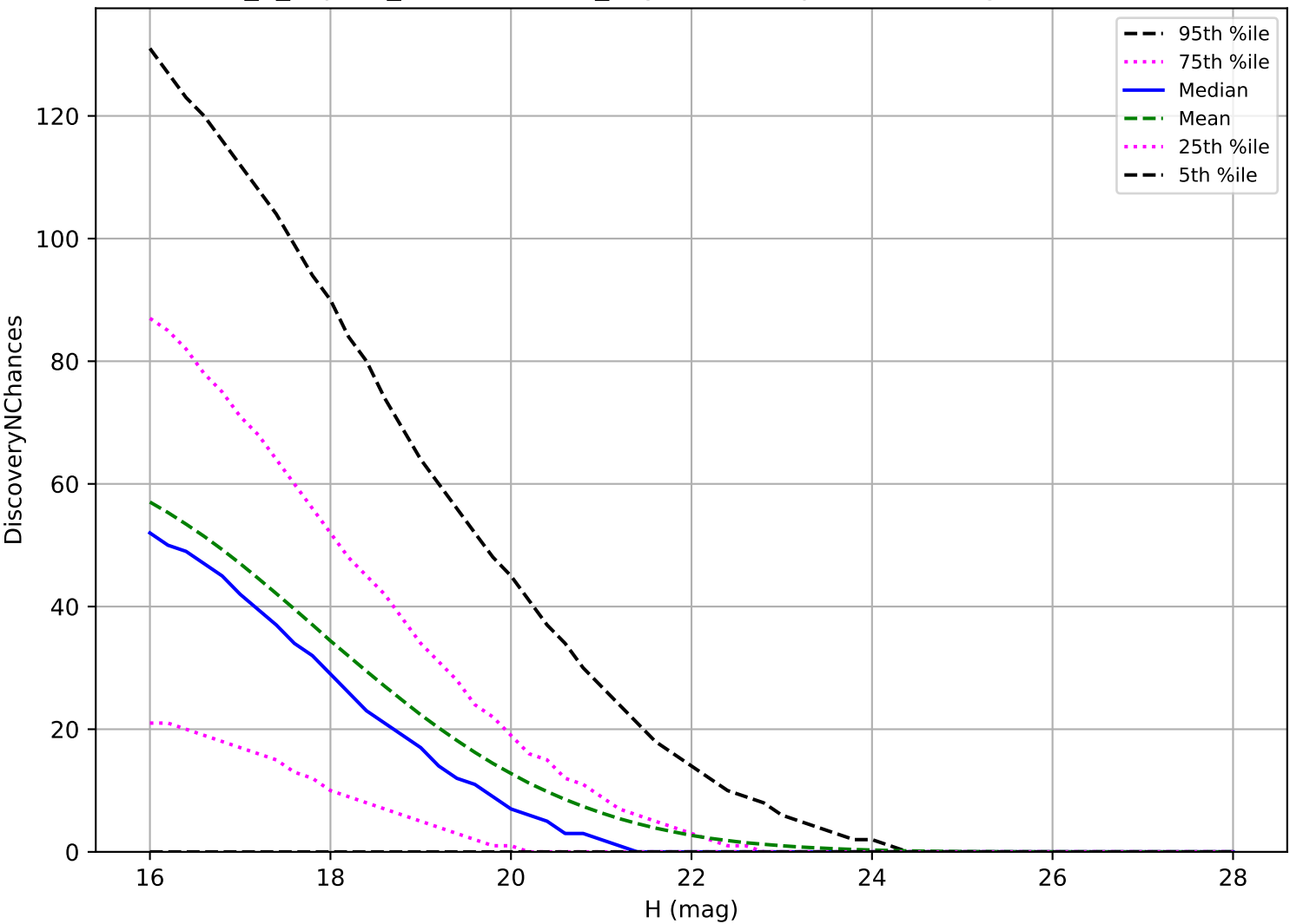
internal_u_expt27_nscale1.1v3.4_10yrs: NEO 3 pairs in 15 nights detection loss
