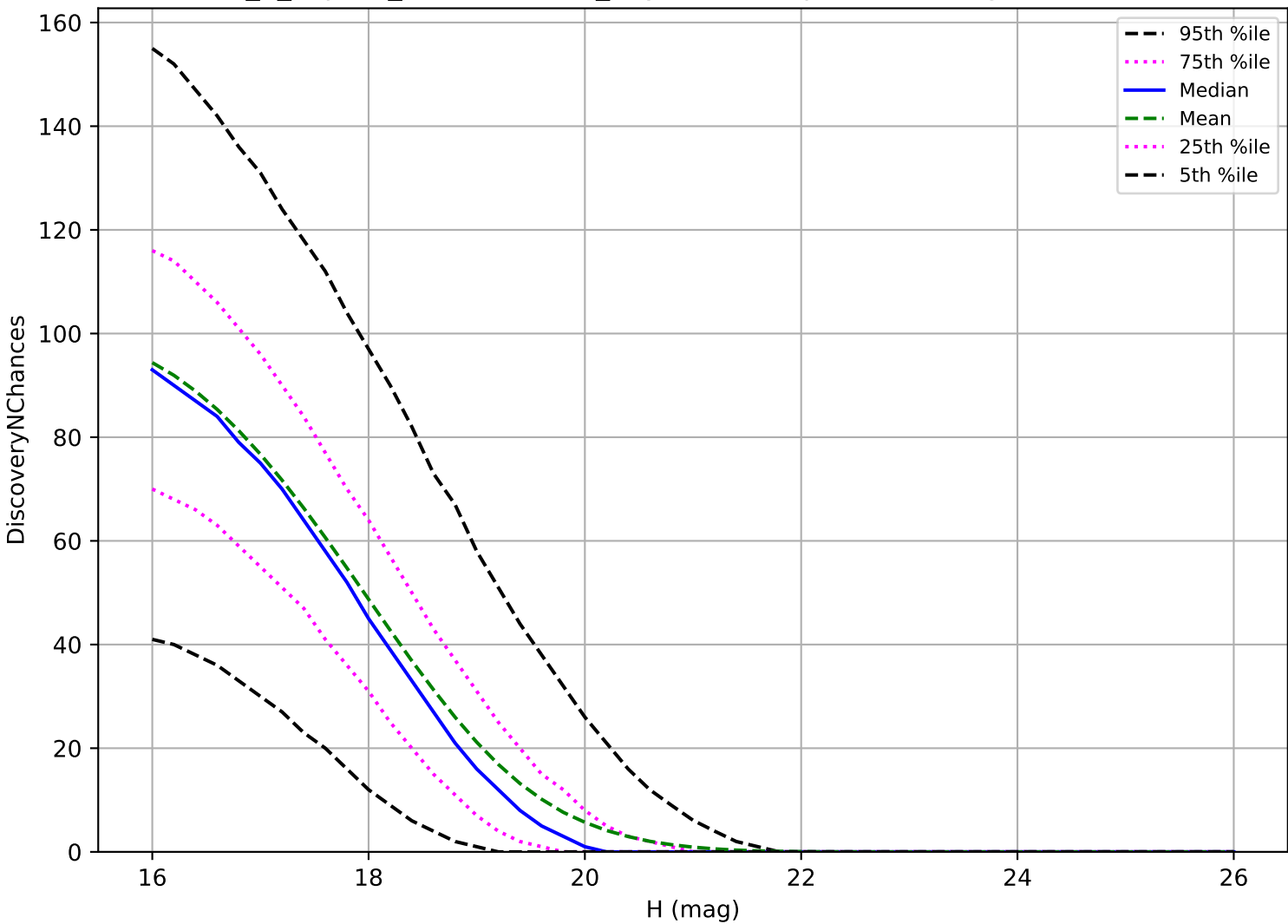
internal_u_expt27_nscale1.1v3.4_10yrs: MBA 3 pairs in 15 nights detection loss
