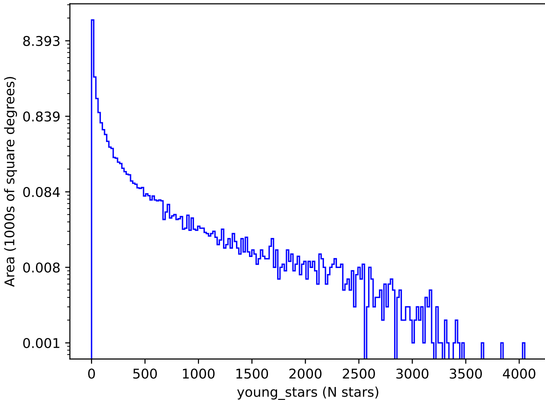
internal_u_expt27_nscale1.1v3.4_10yrs : young_stars
