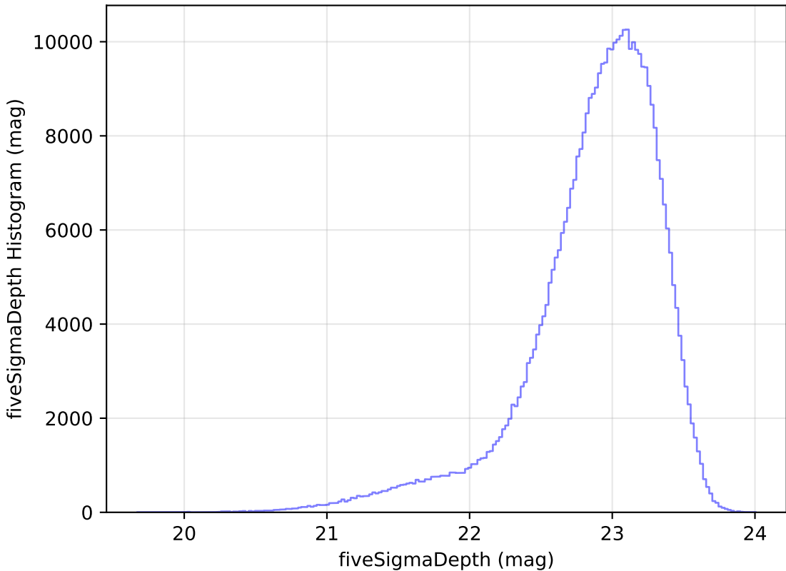
internal_u_expt27_nscale1.1v3.4_10yrs z: fiveSigmaDepth Histogram
