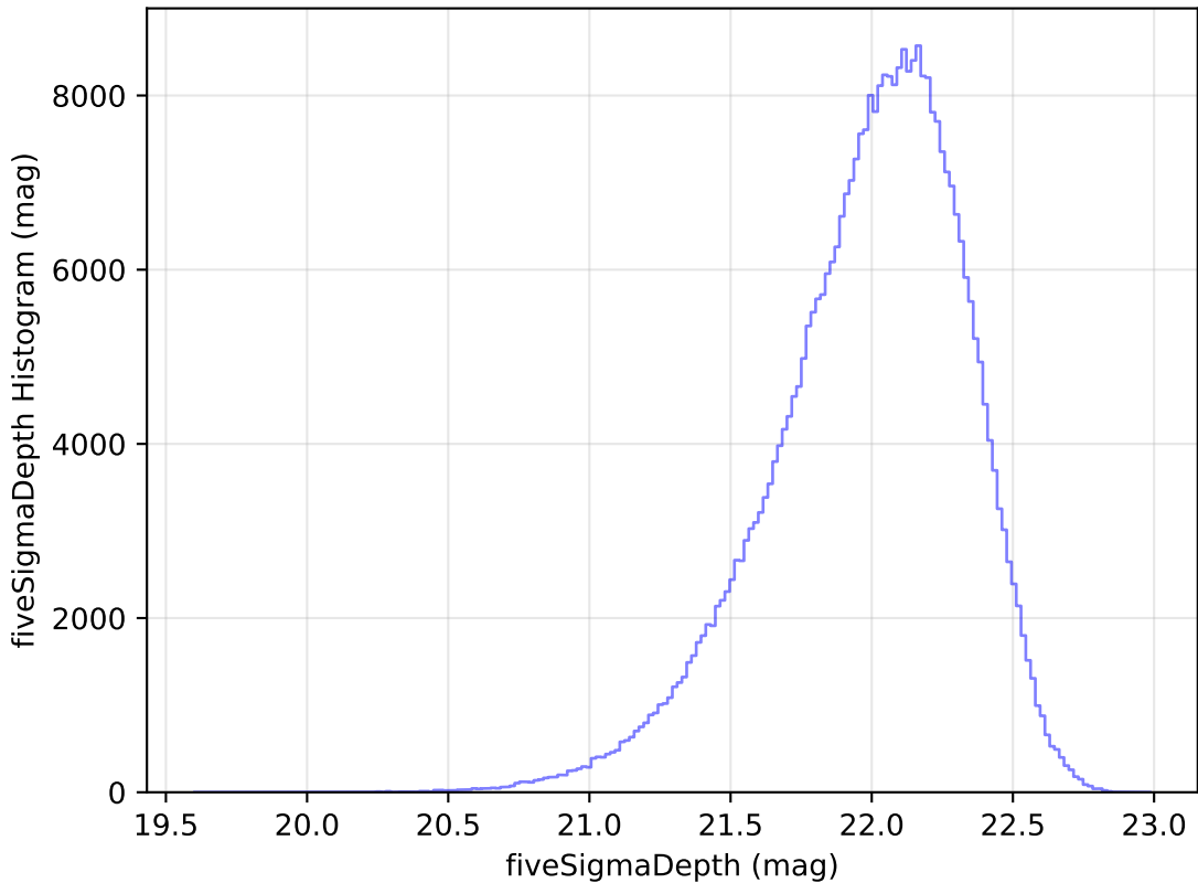
internal_u_expt27_nscale1.1v3.4_10yrs y: fiveSigmaDepth Histogram
