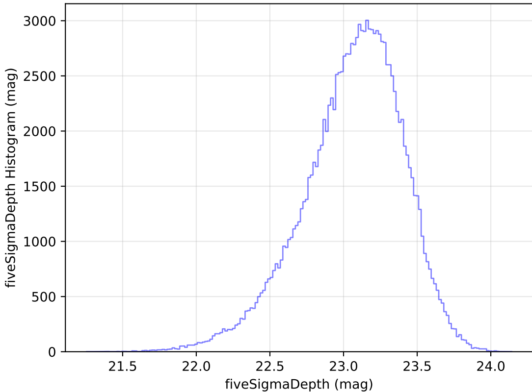
internal_u_expt27_nscale1.1v3.4_10yrs u: fiveSigmaDepth Histogram
