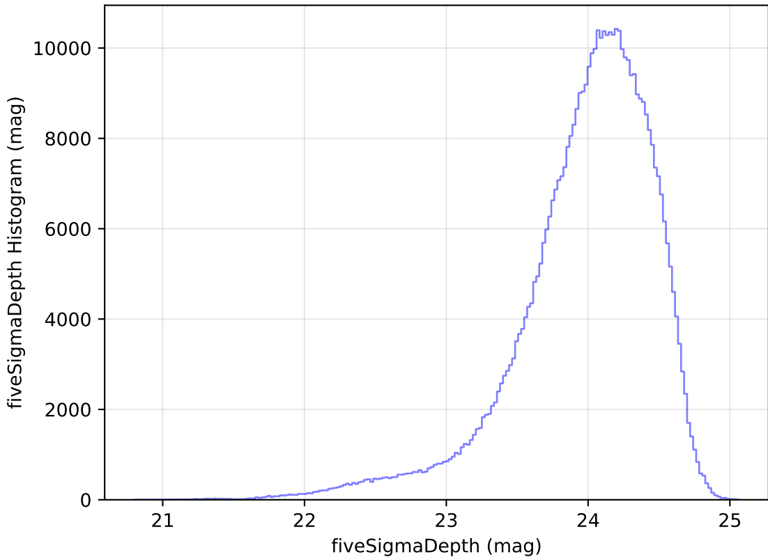
internal_u_expt27_nscale1.1v3.4_10yrs r: fiveSigmaDepth Histogram
