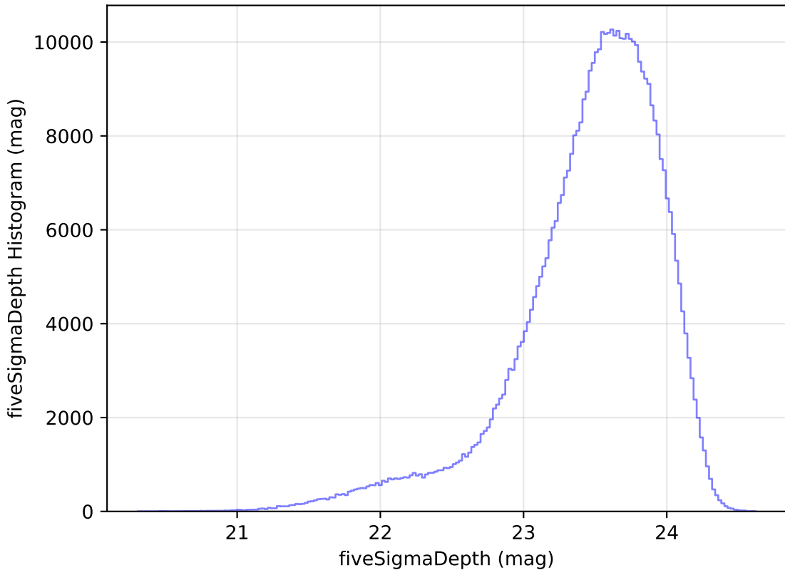
internal_u_expt27_nscale1.1v3.4_10yrs i: fiveSigmaDepth Histogram
