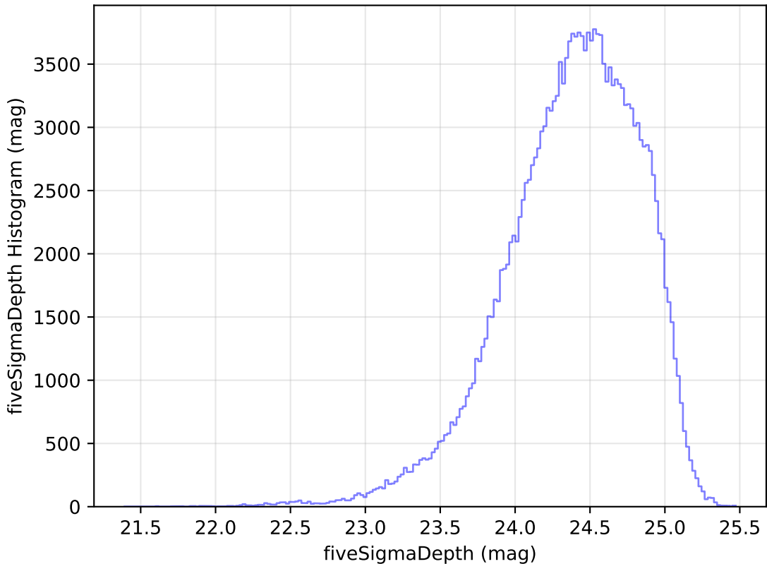
internal_u_expt27_nscale1.1v3.4_10yrs g: fiveSigmaDepth Histogram
