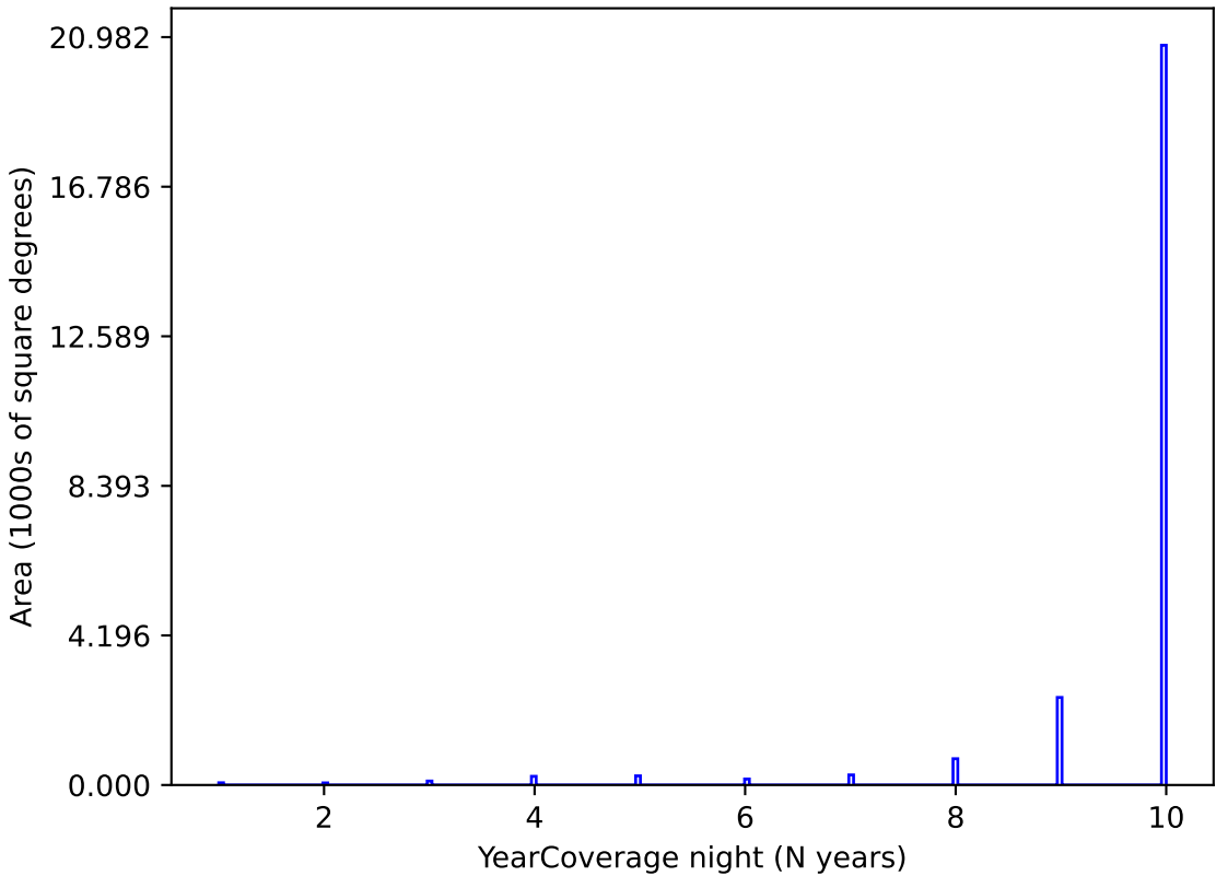
internal_u_expt27_nscale1.1v3.4_10yrs y band: YearCoverage night
