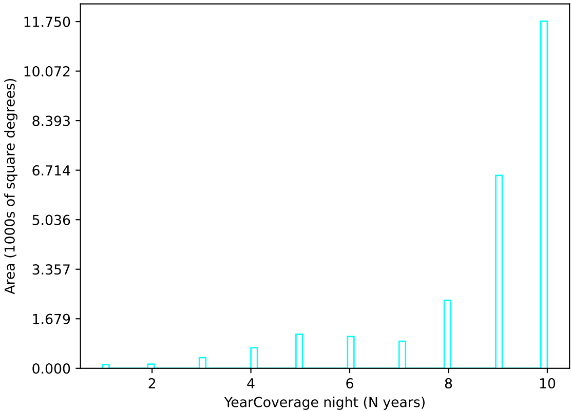
internal_u_expt27_nscale1.1v3.4_10yrs u band: YearCoverage night
