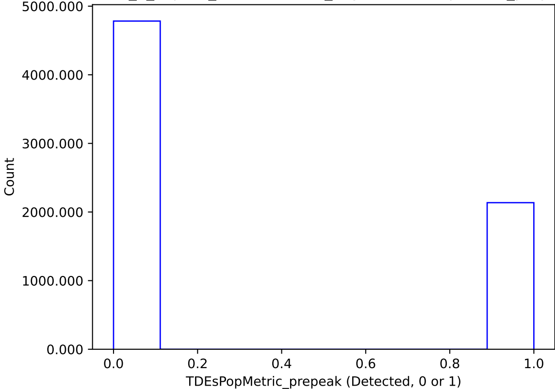
internal_u_expt27_nscale1.1v3.4_10yrs : TDEsPopMetric_prepeak
