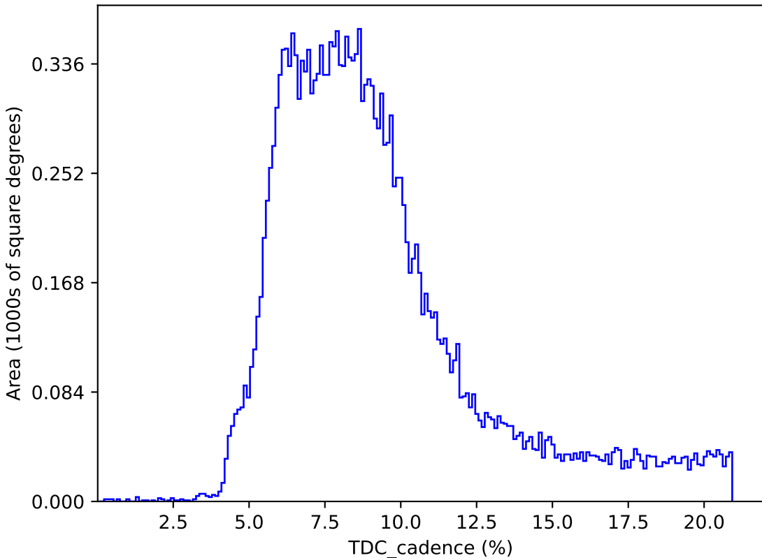
internal_u_expt27_nscale1.1v3.4_10yrs : TDC_cadence
