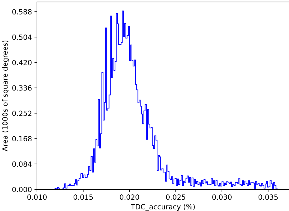
internal_u_expt27_nscale1.1v3.4_10yrs : TDC_accuracy
