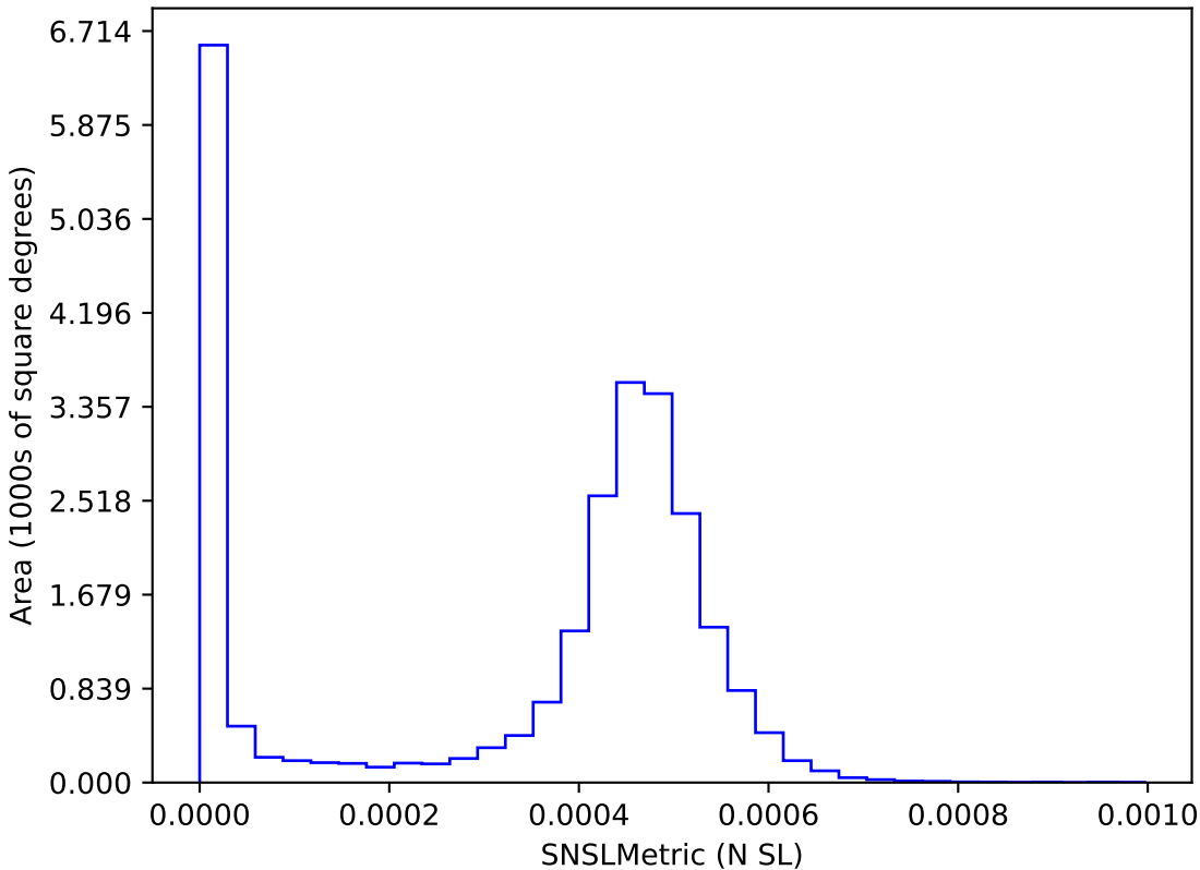
internal_u_expt27_nscale1.1v3.4_10yrs : SNSLMetric
