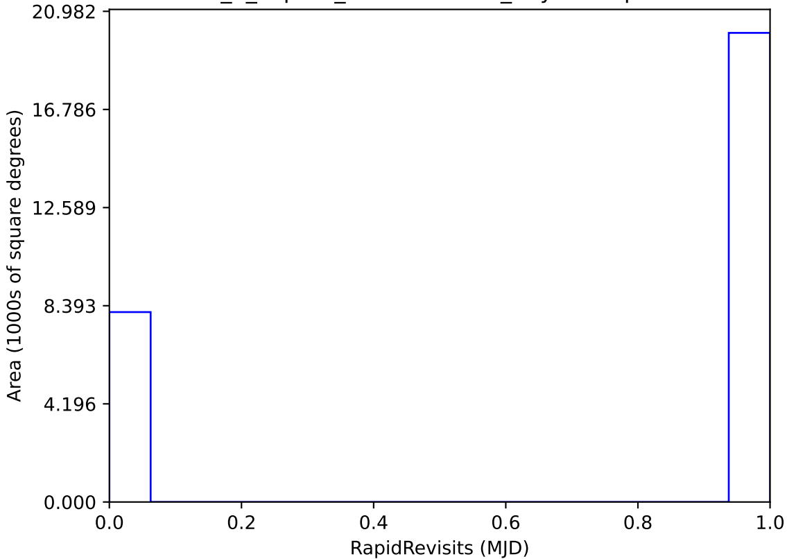
internal_u_expt27_nscale1.1v3.4_10yrs : RapidRevisits
