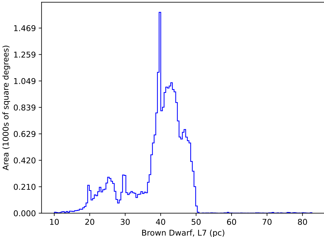
internal_u_expt27_nscale1.1v3.4_10yrs : Brown Dwarf, L7
