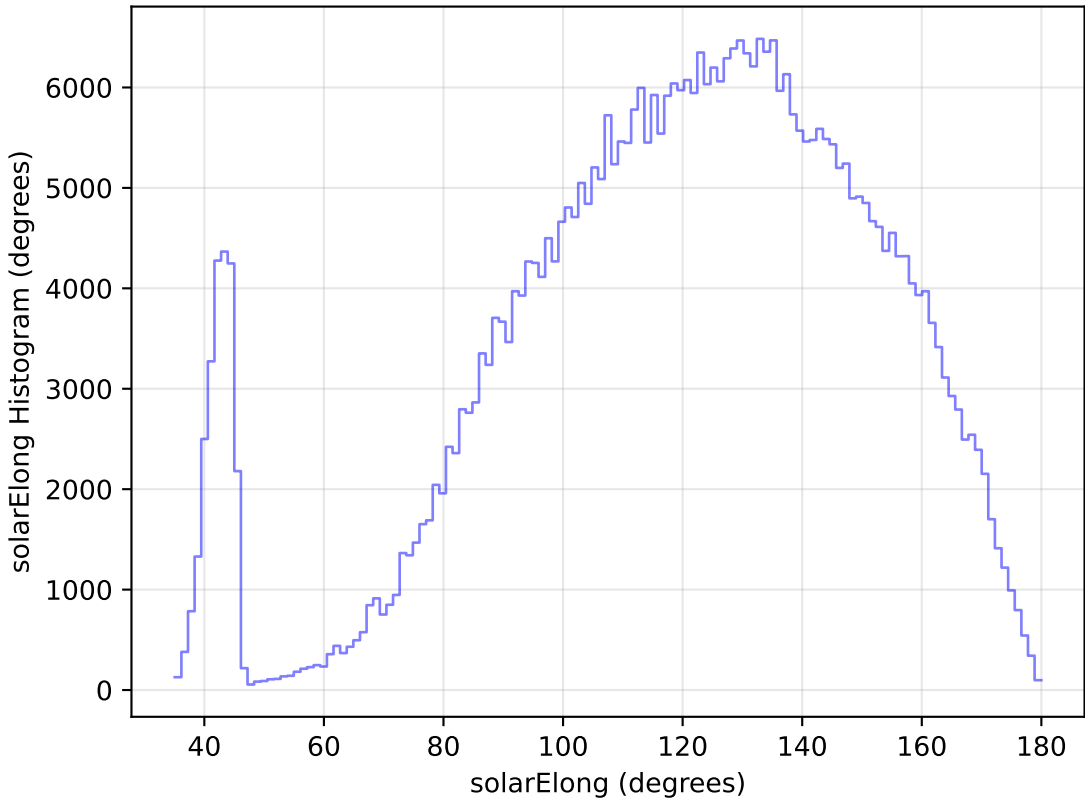
internal_u_expt27_nscale1.1v3.4_10yrs WFD z band: solarElong Histogram
