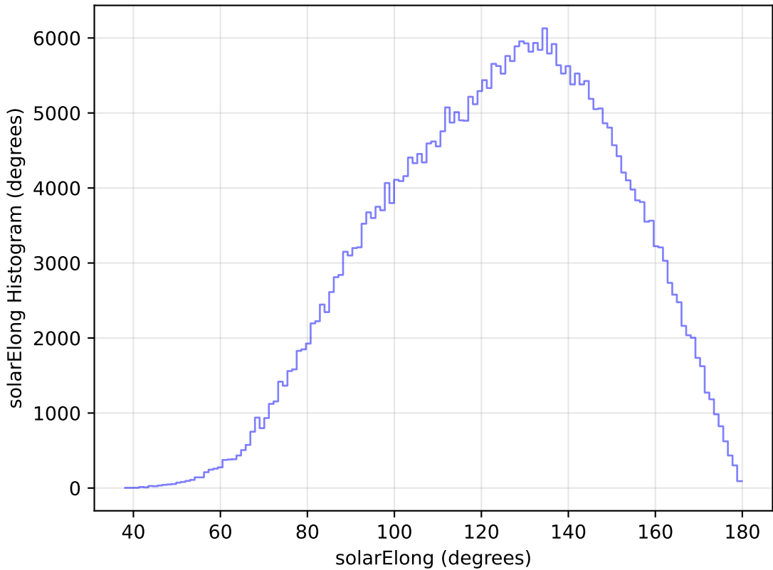
internal_u_expt27_nscale1.1v3.4_10yrs WFD y band: solarElong Histogram
