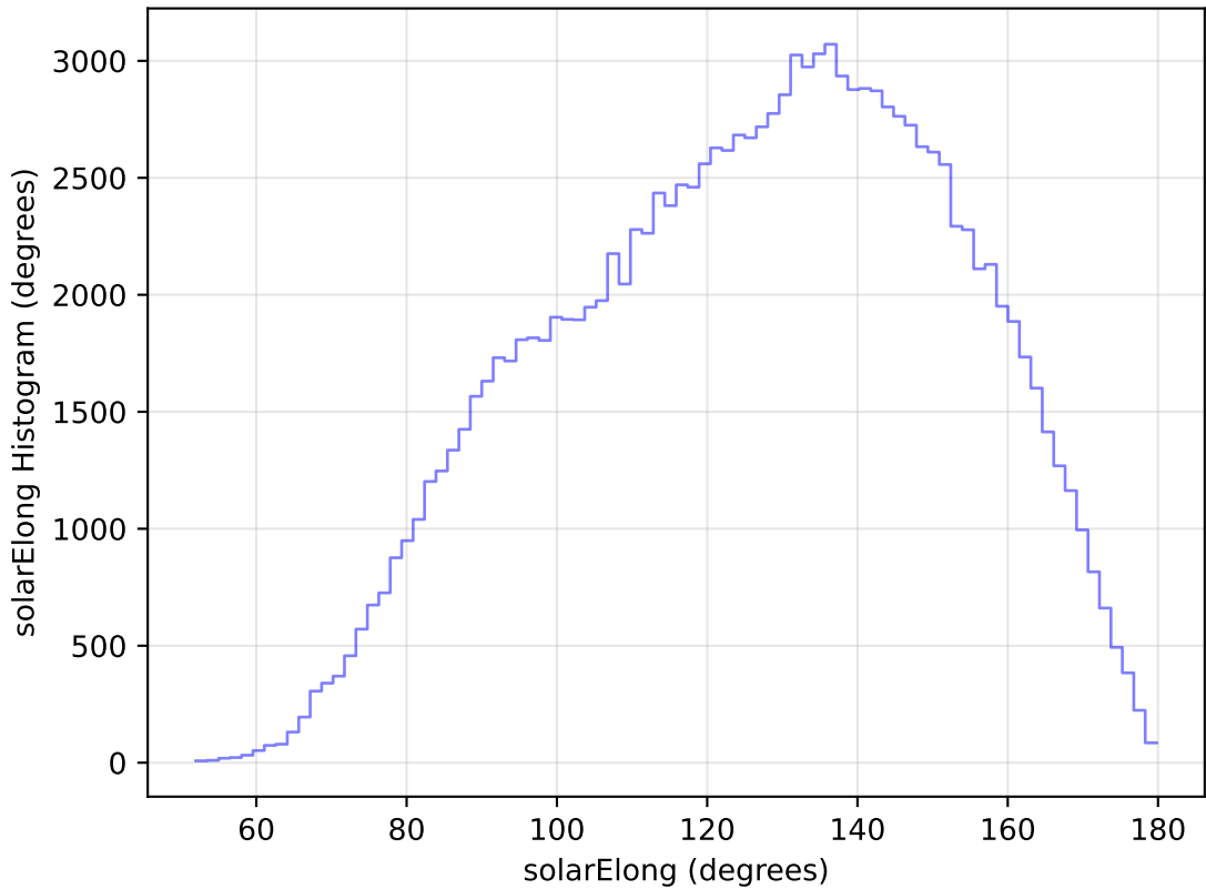
internal_u_expt27_nscale1.1v3.4_10yrs WFD u band: solarElong Histogram
