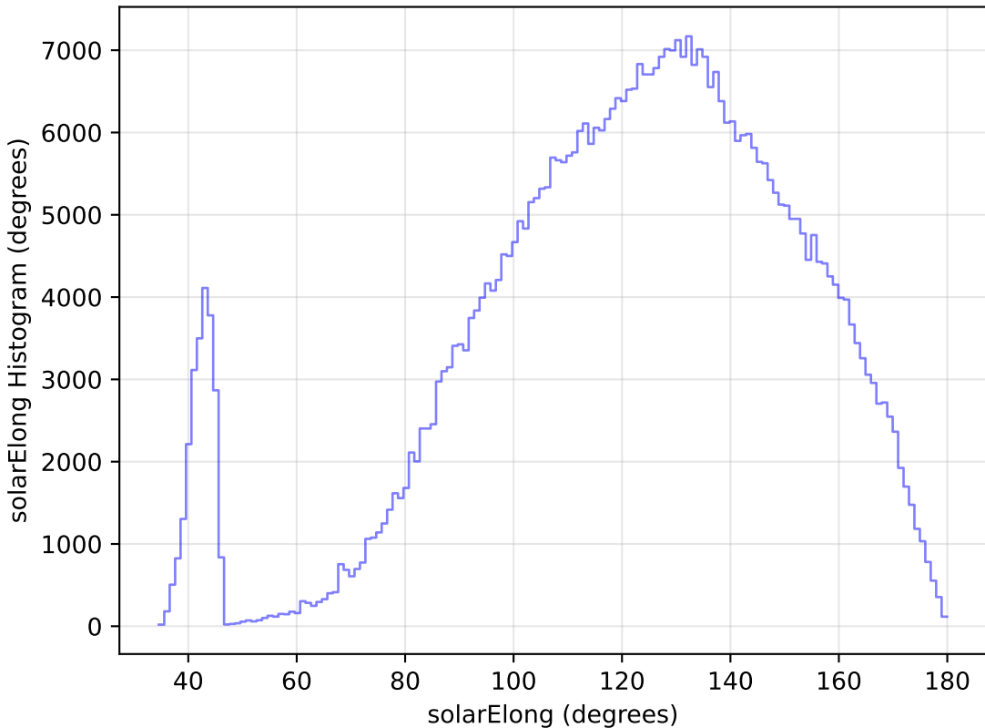
internal_u_expt27_nscale1.1v3.4_10yrs WFD i band: solarElong Histogram
