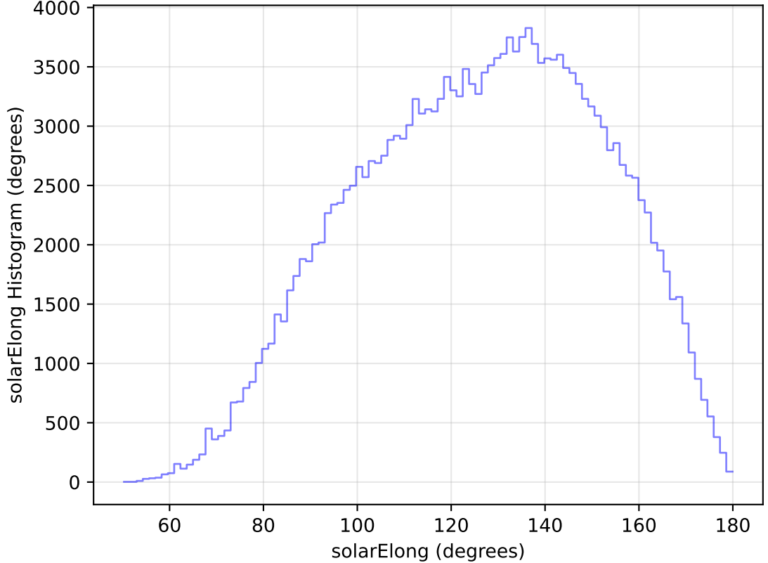
internal_u_expt27_nscale1.1v3.4_10yrs WFD g band: solarElong Histogram
