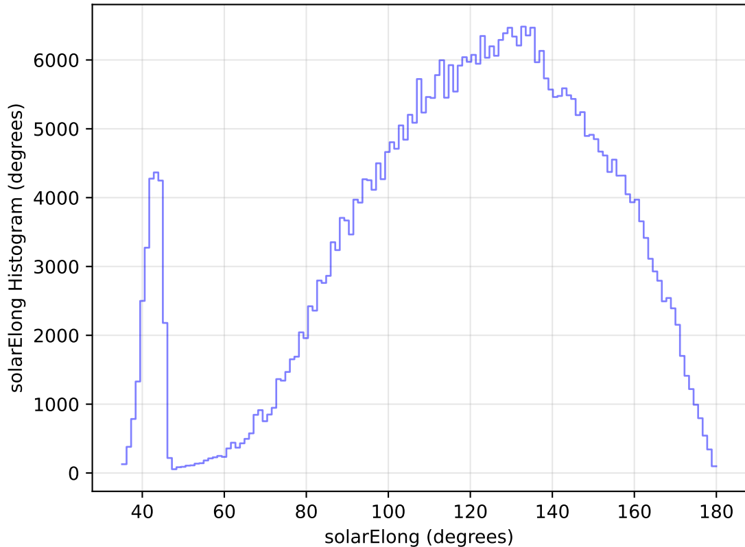
internal_u_expt27_nscale1.1v3.4_10yrs All sky z band: solarElong Histogram
