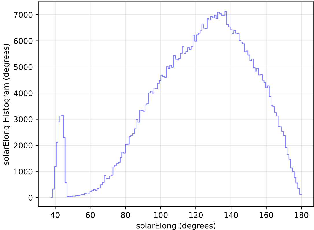
internal_u_expt27_nscale1.1v3.4_10yrs All sky r band: solarElong Histogram
