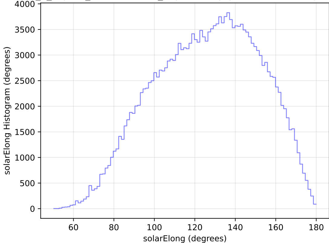
internal_u_expt27_nscale1.1v3.4_10yrs All sky g band: solarElong Histogram
