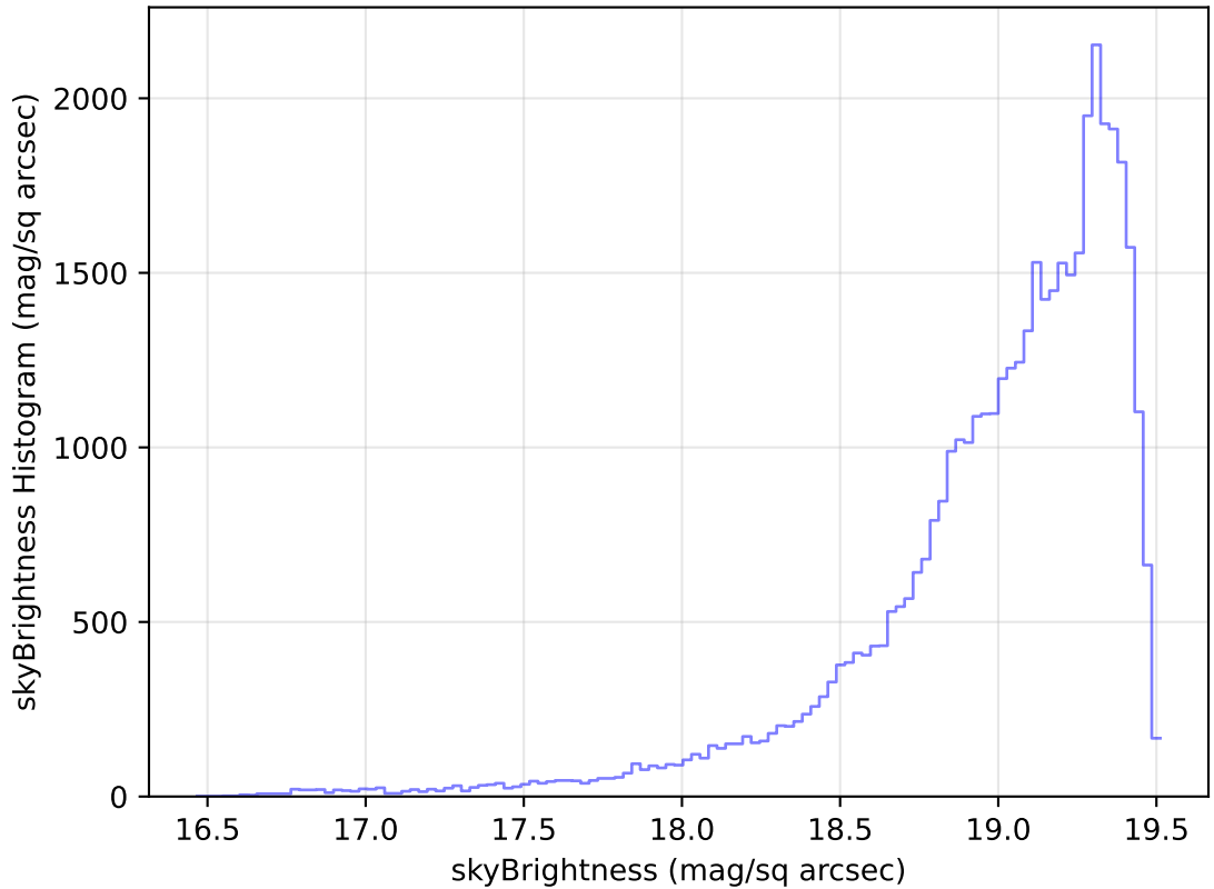
internal_u_expt27_nscale1.1v3.4_10yrs Yr 1 z band: skyBrightness Histogram
