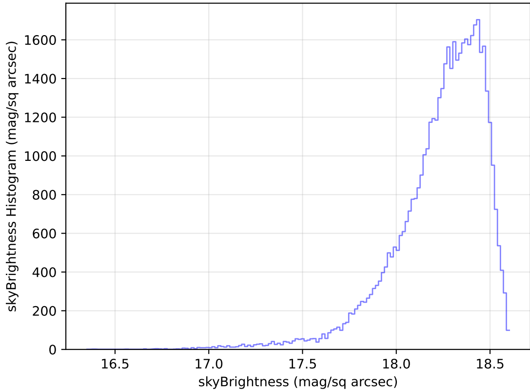
internal_u_expt27_nscale1.1v3.4_10yrs Yr 1 y band: skyBrightness Histogram
