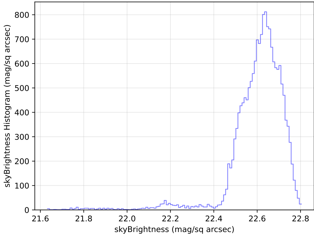
internal_u_expt27_nscale1.1v3.4_10yrs Yr 1 u band: skyBrightness Histogram
