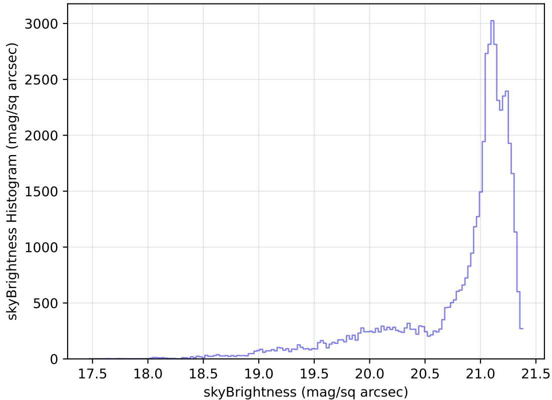
internal_u_expt27_nscale1.1v3.4_10yrs Yr 1 r band: skyBrightness Histogram
