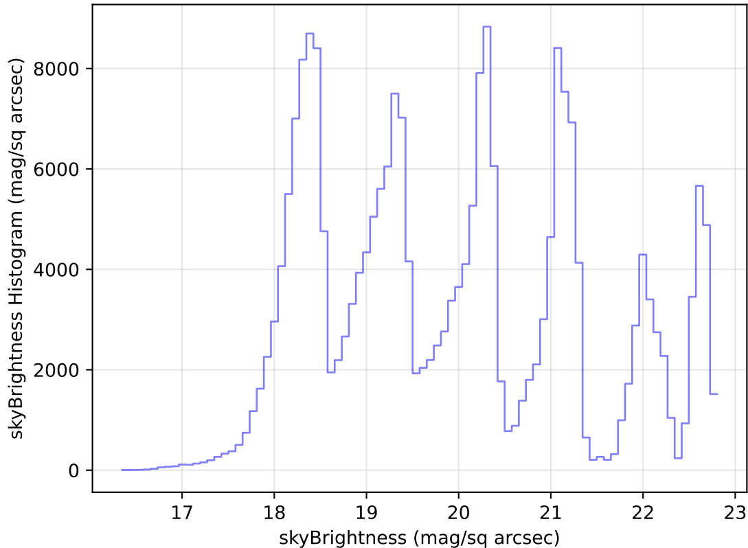
internal_u_expt27_nscale1.1v3.4_10yrs Yr 1 all bands: skyBrightness Histogram
