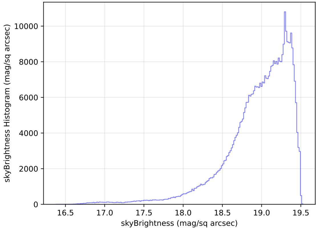
internal_u_expt27_nscale1.1v3.4_10yrs WFD z band: skyBrightness Histogram
